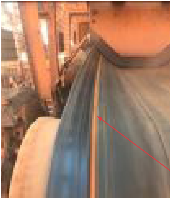
Photo: Typical groove caused by product build-up in skirted section.
