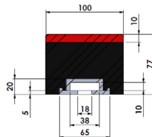
77 x 100 x 1400mm Standard Impact Bar
